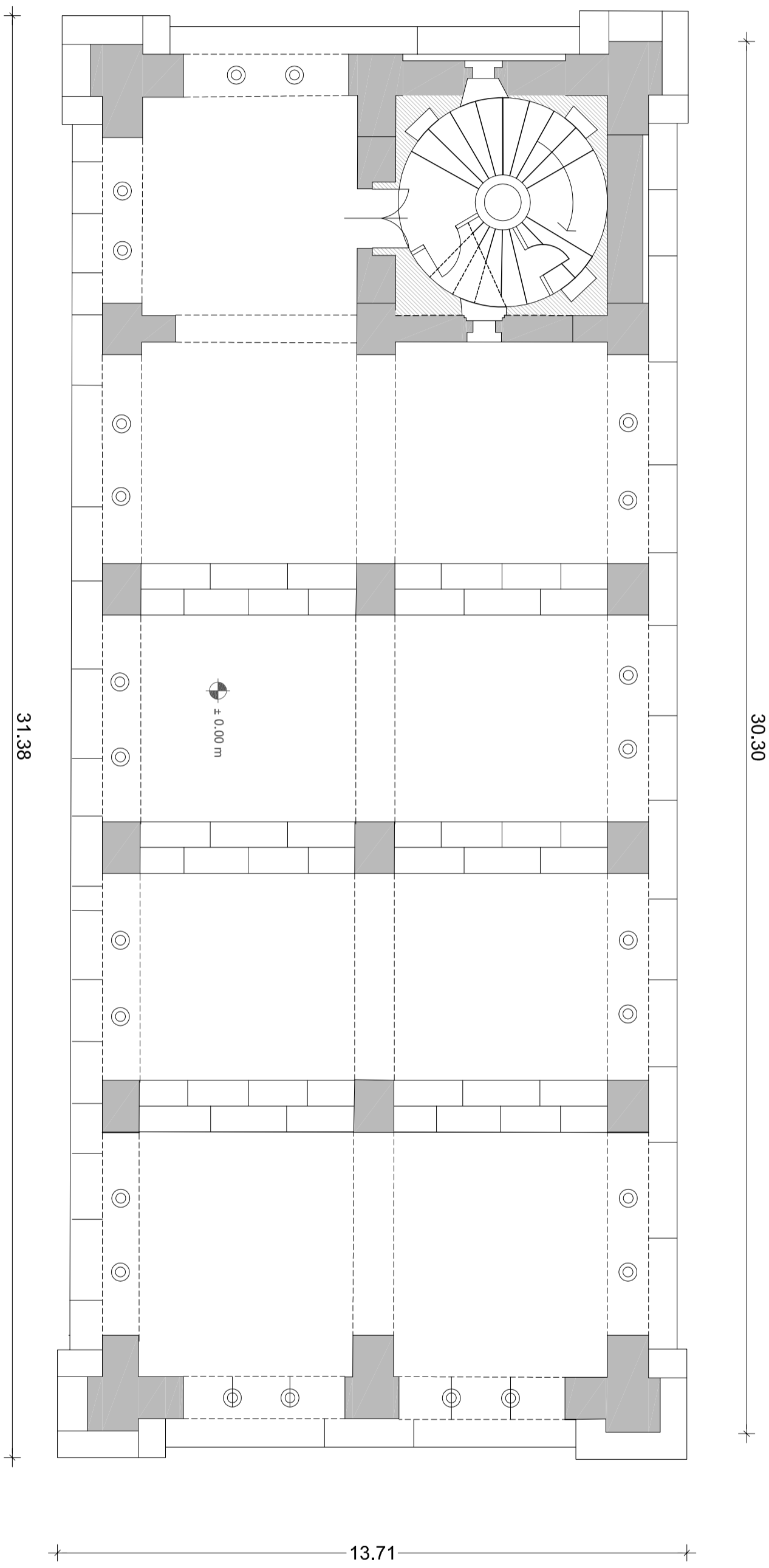
PIANTA PIANO TERRA ± 0.00 m
